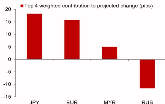
Fig. 1: Top 4 weighted overnight contribution to projected change (without counter-cyclical factor)
