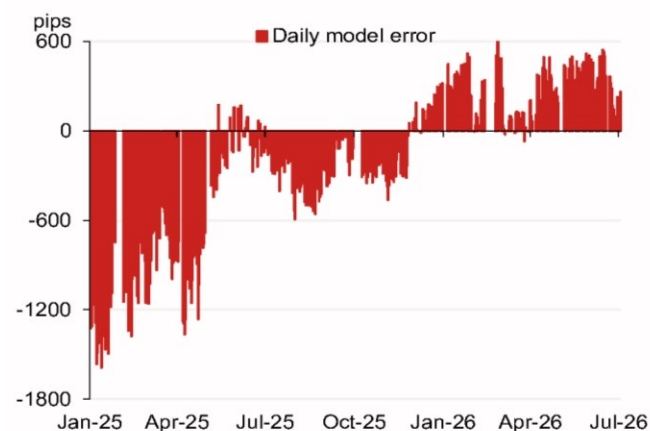
Fig. 2: Recent model errors (without counter-cyclical factor adjustment)
