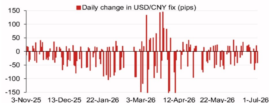
Fig. 3: Daily change in USD/CNY fix
