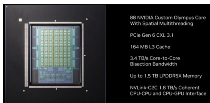
Exhibit 6: Vera CPU cores are not split across chiplets, enabling faster core-to-core connection
