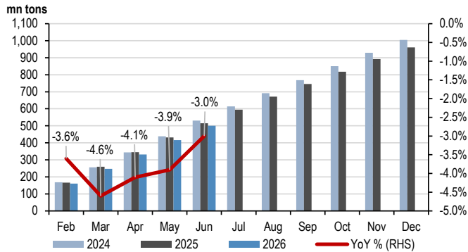
Figure 11: China YTD Crude Steel Production
