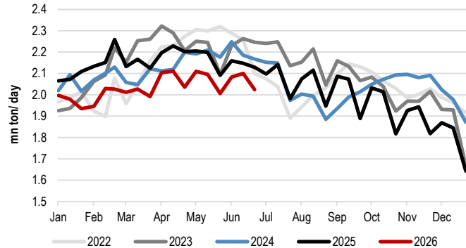
Figure 12: CISA Key Members Daily Average Crude Steel Output
