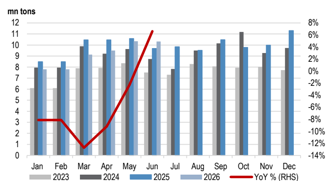
Figure 16: China Steel Products Export Volume
