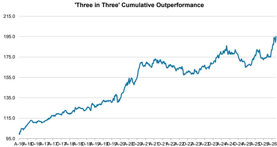
Exhibit 2: Cumulative outperformance
