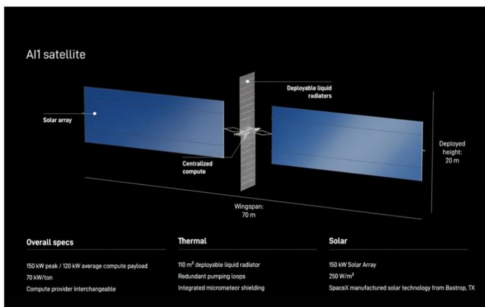
Figure 1 - Figure 1: SpaceX AI1 satellite design
