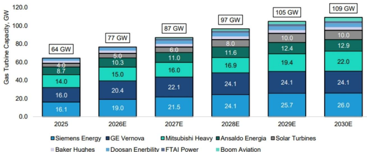
EXHIBIT 14 - EXHIBIT 15: There has never been a better time to be a manufacturer of natural gas turbines. Gas turbine orders are set to increase to 100GW annually in the next few years which outpace current capacity of 60GW Global gas turbine or
