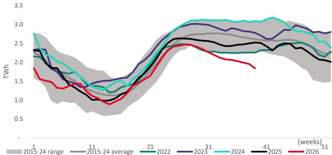
EXHIBIT 11 - EXHIBIT 11: French hydropower production EXHIBIT 12: French water reservoir and hydro storage levels (TWh) ## TOTAL PRODUCTION EXHIBIT 13: France's power production (TWh)
