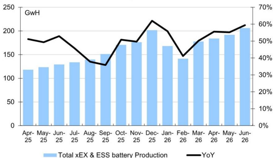
Figure 3 - Figure 4: China xEV and ESS battery production volume trend Figure 5: China xEV and ESS battery production volume trend by product
