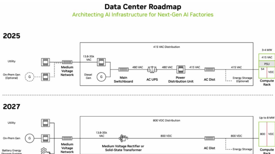
Figure 1 - © 2026 Citi Inc. No redistribution without Citi's written permission. Update of new product 10kV commercial solid-state transformer ('SST') for 800V high-voltage DC AI data centers - Sungrow signed orders with two domestic buyers when it launched its SST new p
