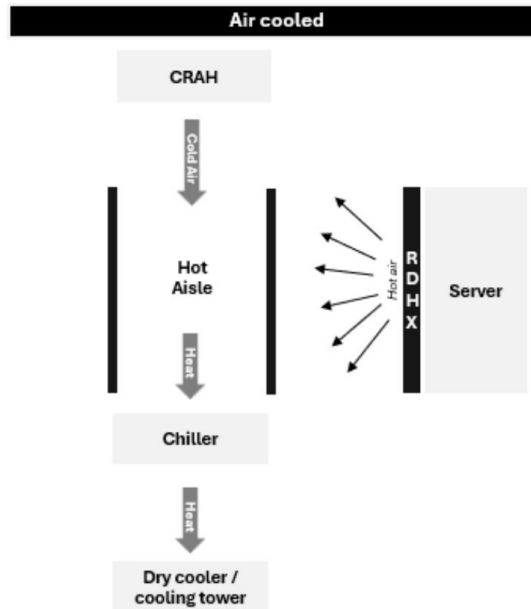
EXHIBIT 3 - EXHIBIT 3: Different cooling architectures for data centers Heat dumped externally outside facility Heat dumped externally outside facility EXHIBIT 4: Components needed for cooling in data centers (1/2)
