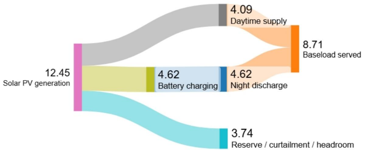
EXHIBIT 5 - EXHIBIT 5: Annual power output of the project (TWh). Solar and storage overbuilt enables continuous 1 GW output
