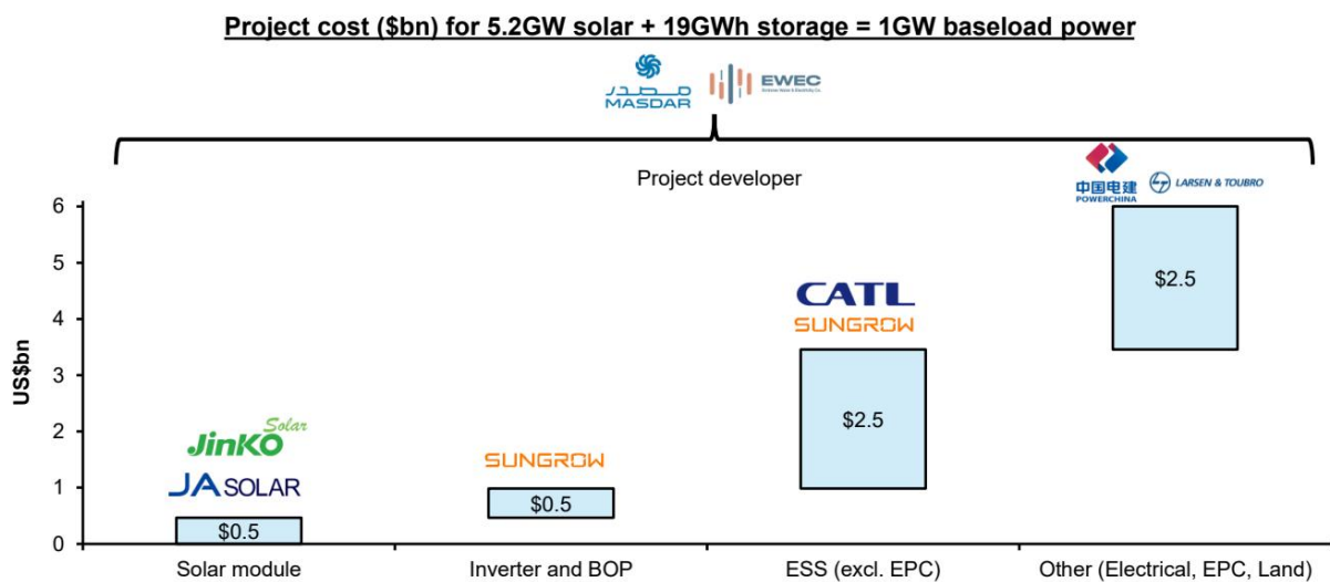
EXHIBIT 2 - EXHIBIT 2: We estimate total project capex at approximately $6bn (or ~$6,000/kW). Energy storage dominates the economics Project cost ($bn) for 5.2GW solar + 19GWh storage = 1GW baseload power
