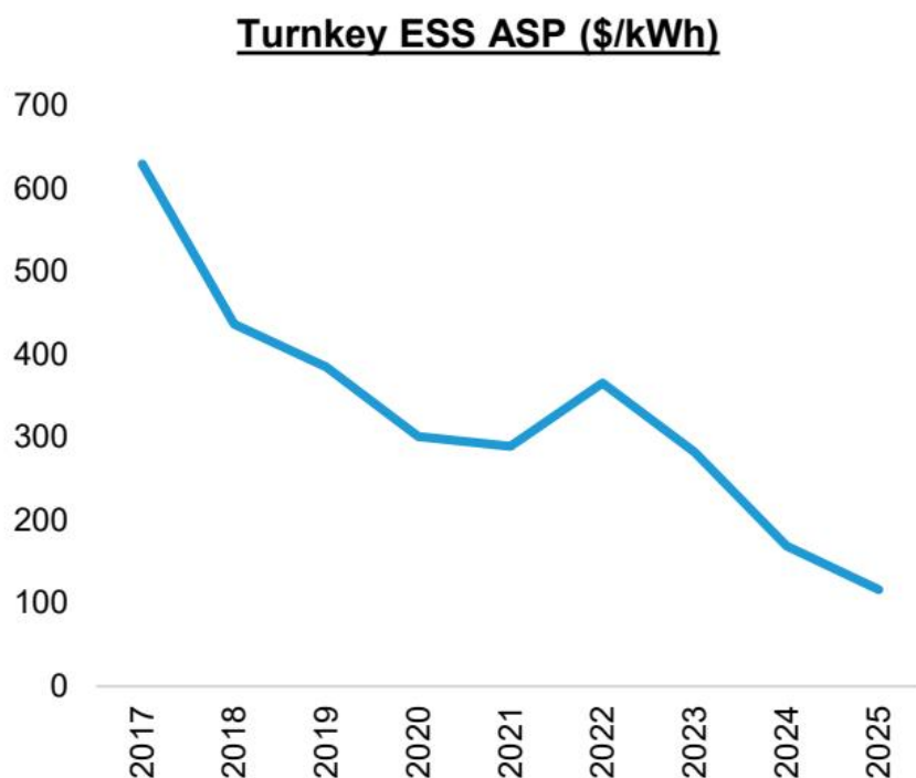
EXHIBIT 16 - EXHIBIT 16: ESS costs have also continued to decline in recent years
