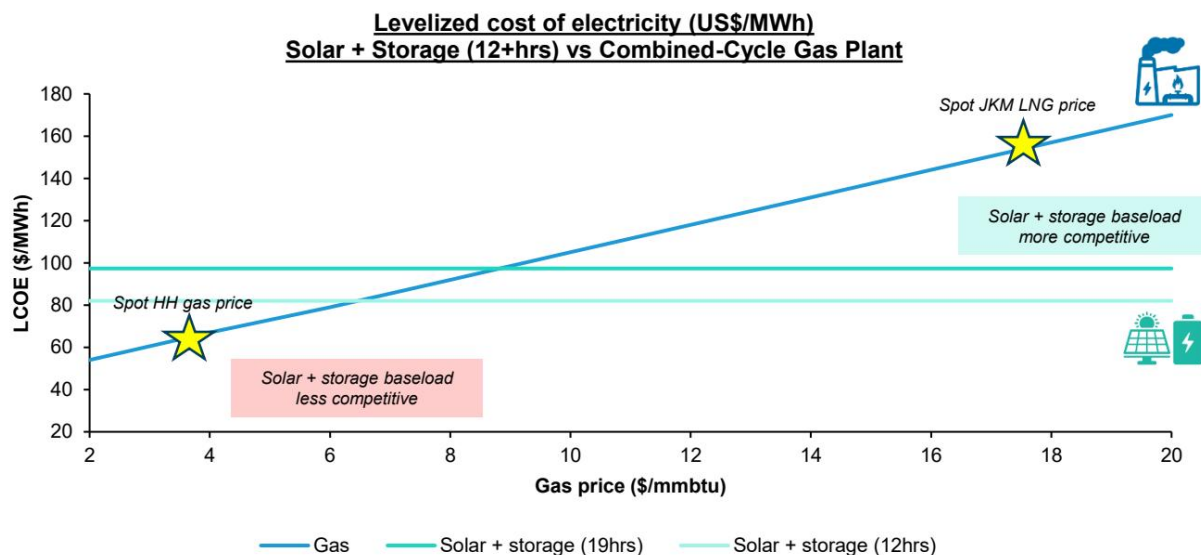
EXHIBIT 1 - EXHIBIT 1: Solar plus storage (12+ hours) are competitive against gas-fired power at high gas prices
