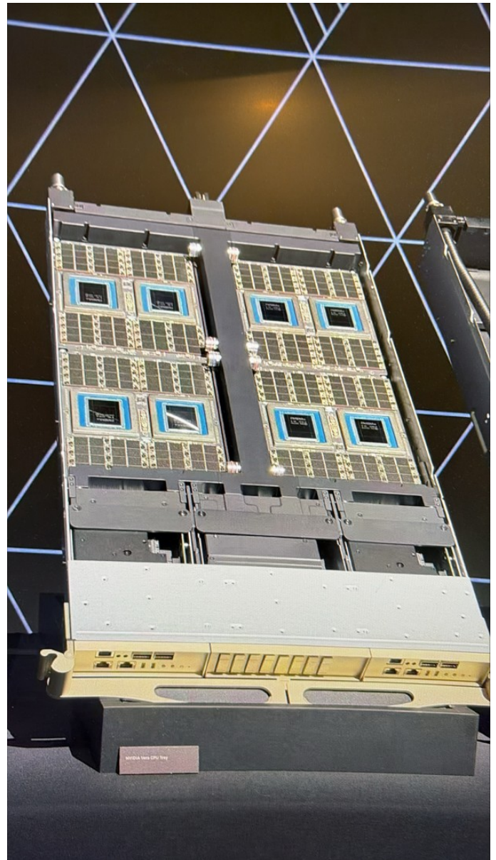
Exhibit 2: Close-up look of a Vera CPU tray
