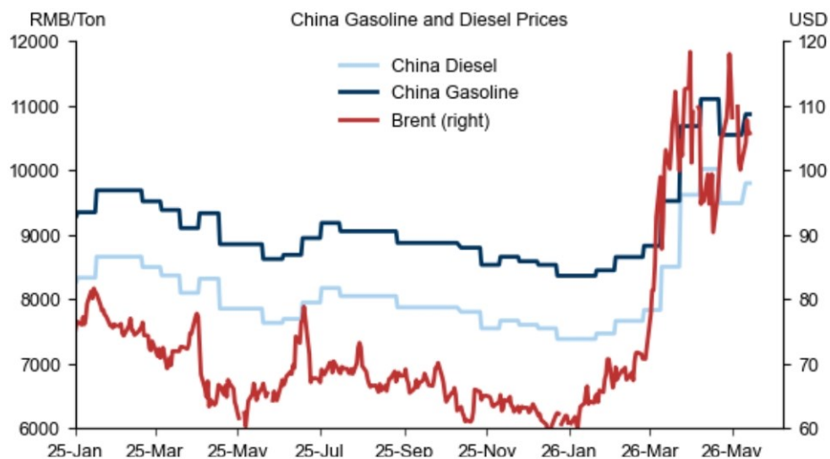
Exhibit 6: Domestic gasoline and diesel prices were raised by 320 and 310 RMB/tonne respectively on 11 May
