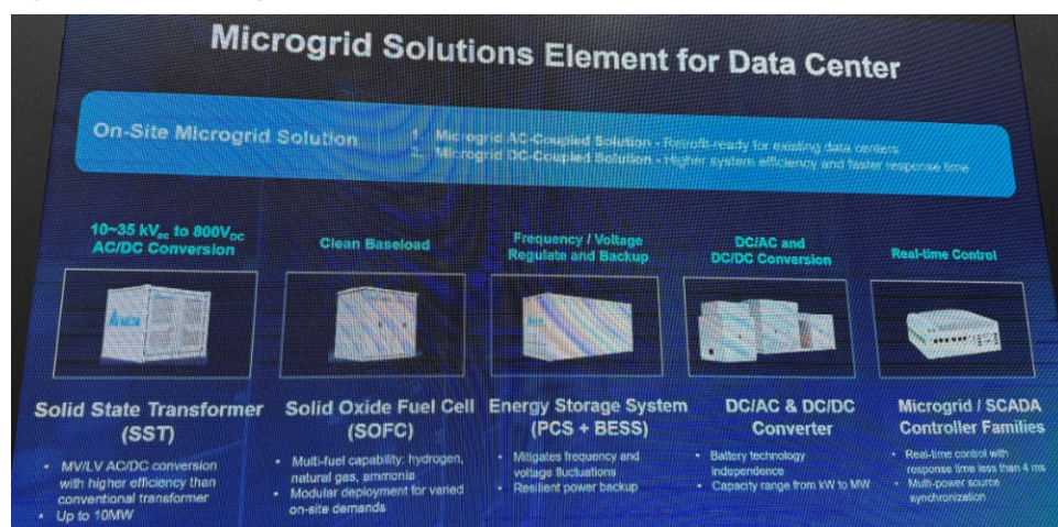
Figure 2: Delta's micro-grid solution elements for datacenter
