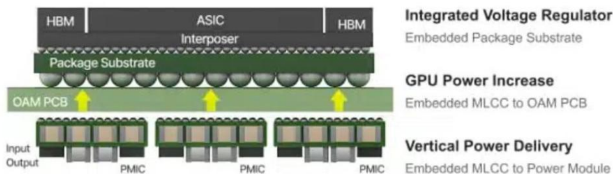
Exhibit 1 - Exhibit 2: MLCC evolution in AI servers
