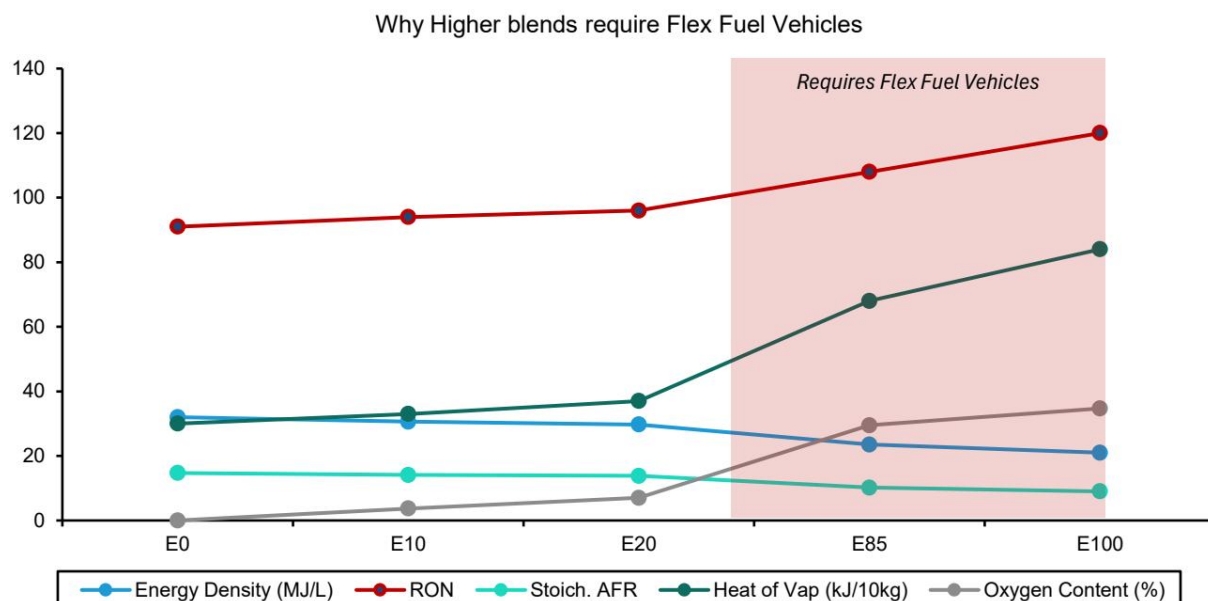
EXHIBIT 2 - EXHIBIT 2: Fuel Properties E0 to E100: The physics are clear - energy density drops from 32 MJ/L at E0 to 21 MJ/L at E100, while the RON rises from 91 to 120. The jump from E20 to E85 is not incremental; it requires entirely new en
