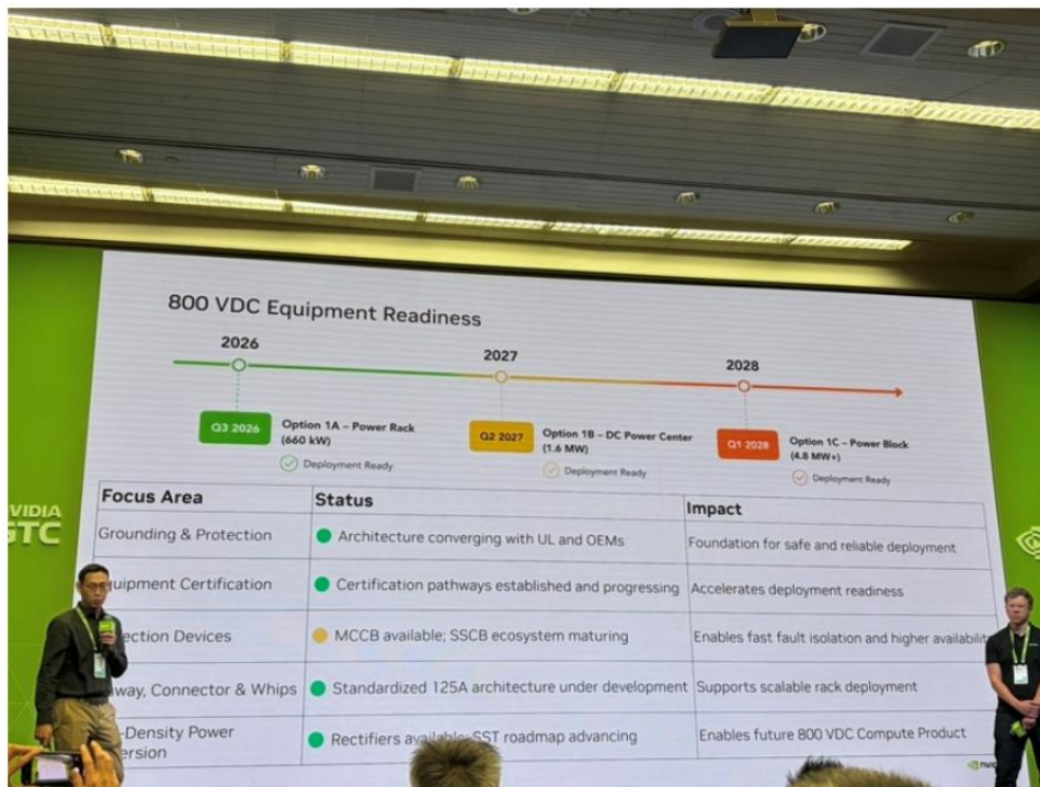
Exhibit 1 - Exhibit 1: 800 VDC equipment readiness 800 VDC Equipment Readiness Q3 2026 Option 1A – Power Rack (660 kW) Q2 2027 Option 1B – DC Power Center (1.6 MW) Q1 2028 Option 1C – Power Block
