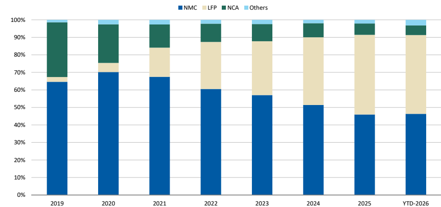
Exhibit 27: % of MWh Deployed by Chemistry
