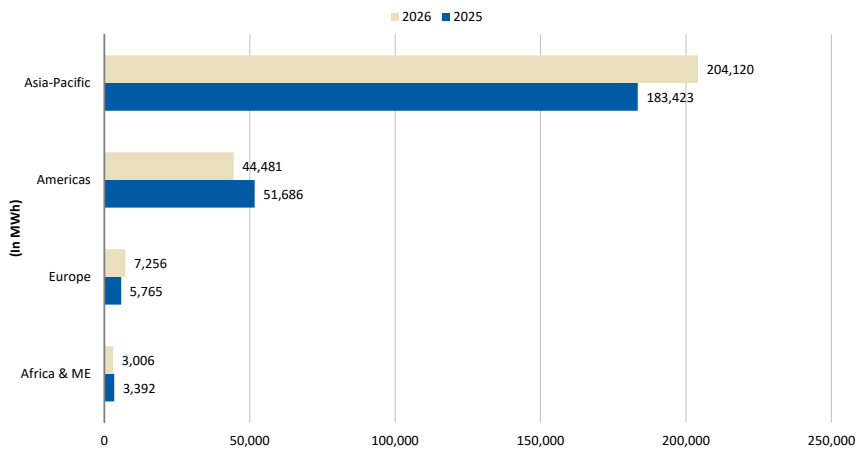
Exhibit 22: May 2026: YTD Deployments by Region in MWh
