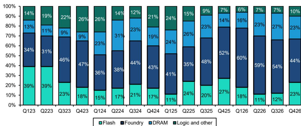
EXHIBIT 2 - EXHIBIT 4: NAND and Logic saw strong growth QoQ, while Foundry and DRAM were down slightly QoQ EXHIBIT 5: Memory share was up 7ppt QoQ to 46% with equal share from DRAM and NAND Lam Research
