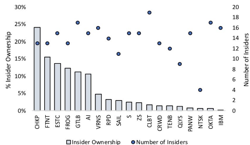
% Insider Ownership
