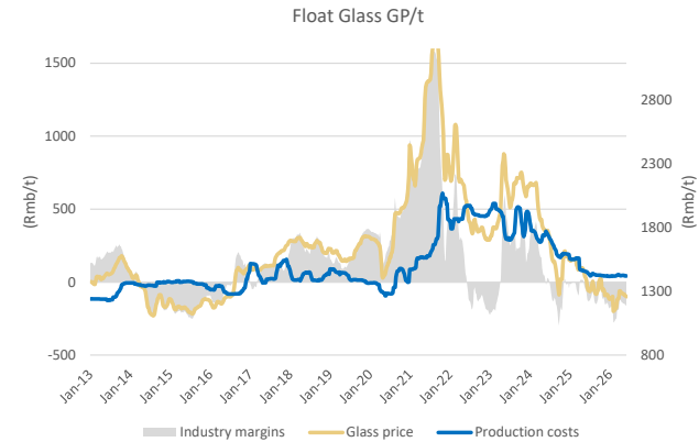
Float Glass Margin
