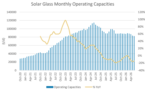
Solar Glass Capacity
