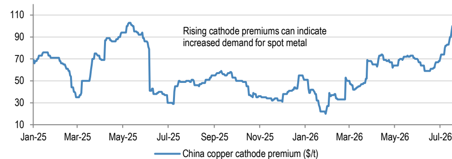
Figure 18: China cathode premium ($/t)
