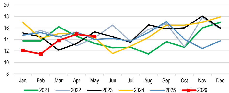
Figure 30: Copper refined + scrap + concentrate net imports (Mtpa rate)
