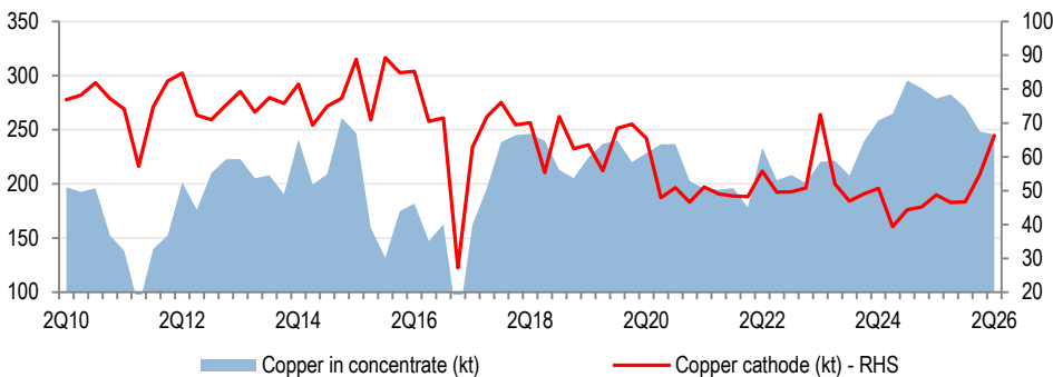
Figure 37: Escondida copper production (kt per quarter)
