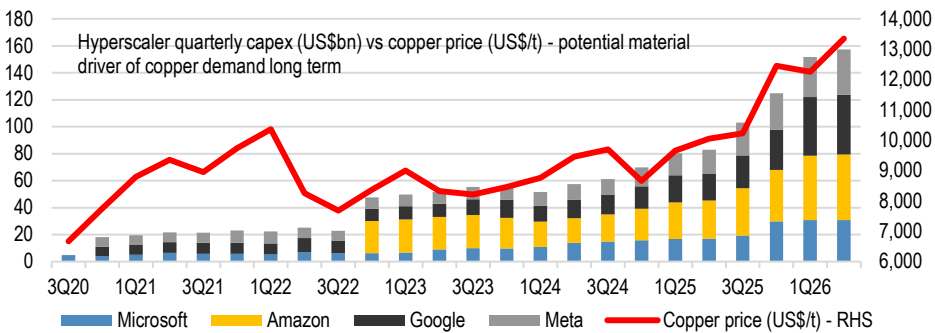
Figure 15: Hyperscaler capex vs copper price (currently datacenter demand is ~400ktpa)
