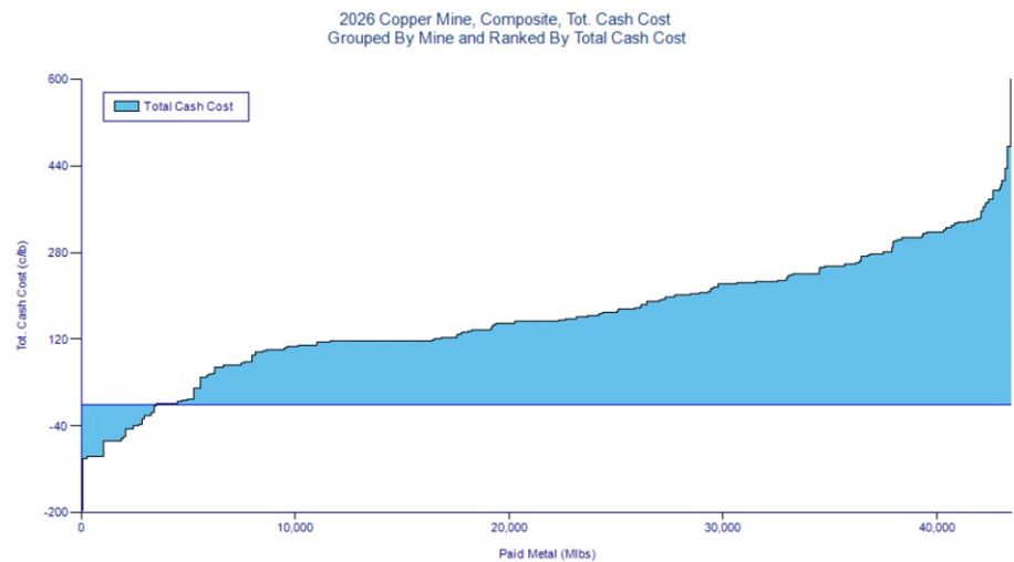
Figure 23: 2026 Copper mine cost curve, ranked by total cash costs
