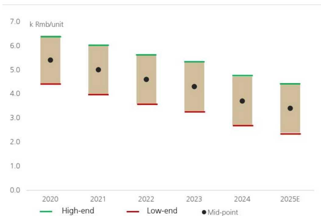
Figure 6 - Figure 6: Cost of SiC substrates, the main production input, has fallen significantly since 2020
