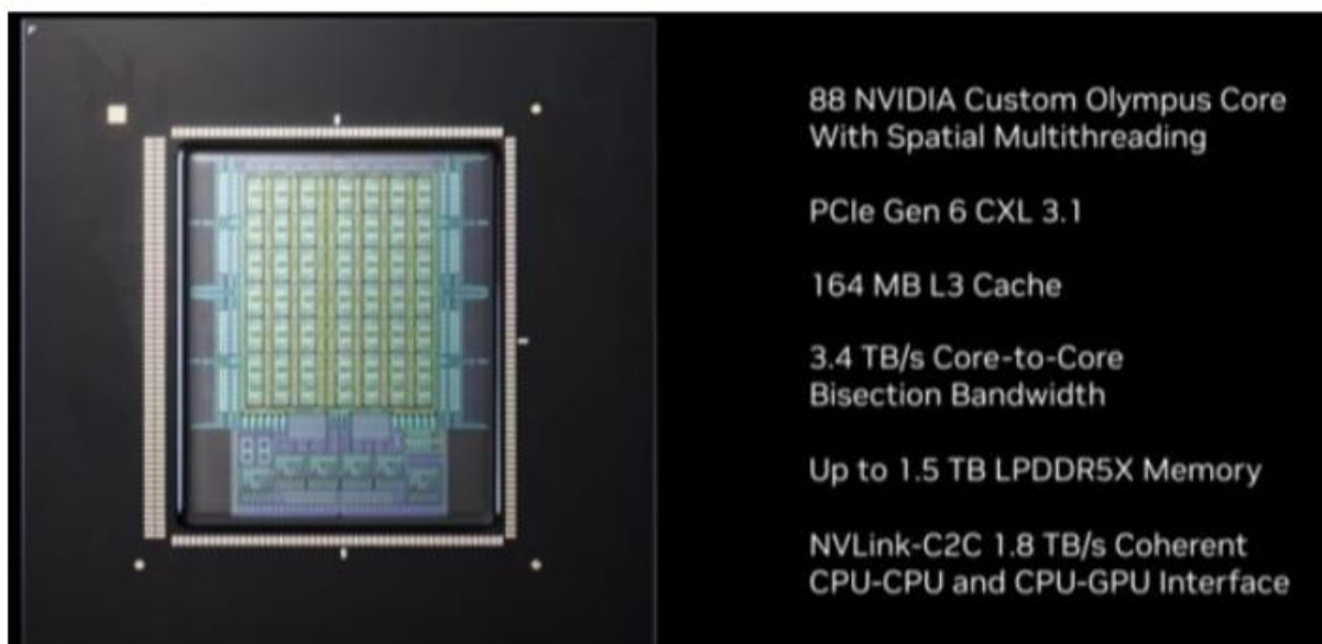
Exhibit 6 - Exhibit 6: Vera CPU cores are not split across chiplets, enabling faster core-to-core connection 88 NVIDIA Custom Olympus Core With Spatial Multithreading PCIe Gen 6 CXL 3.1 164 MB L3 Cache
