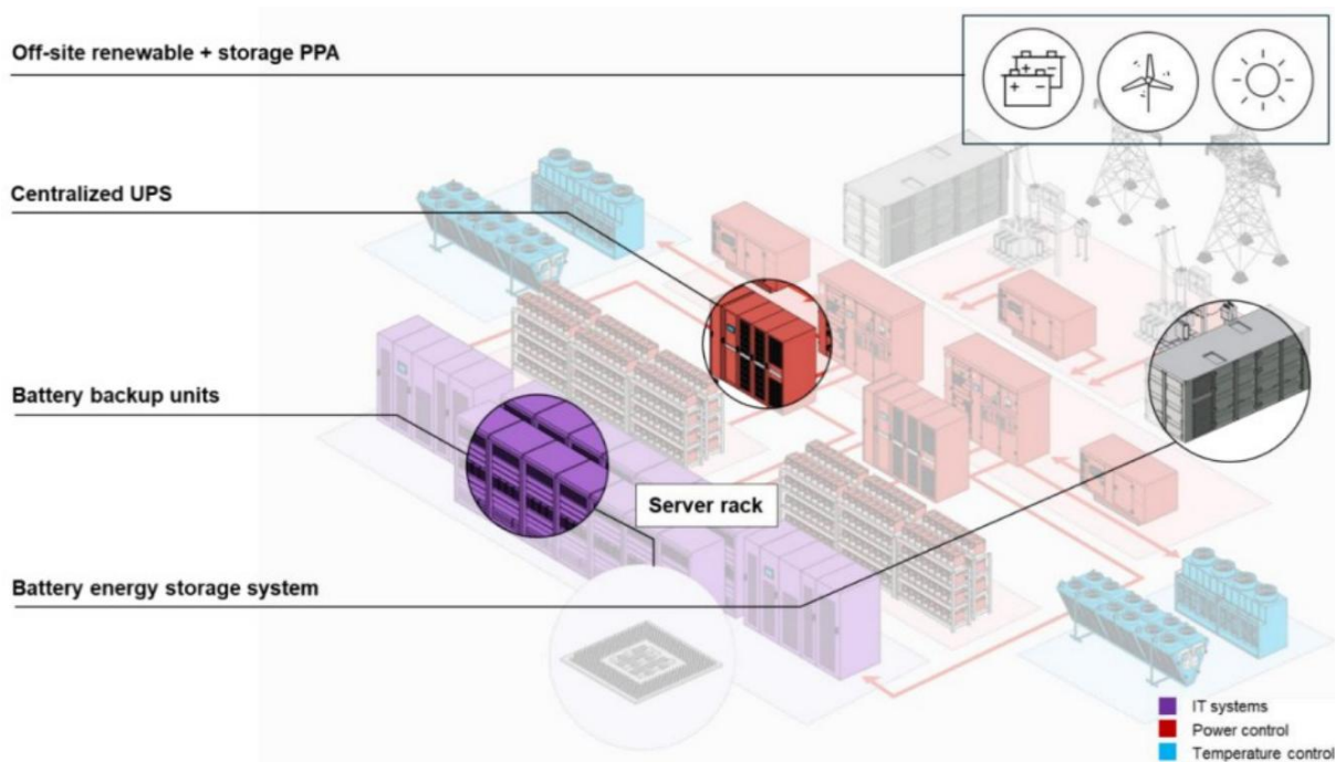
Figure 1 - Figure 1: Levels of energy storage in a data center ""mermaid graph TD
