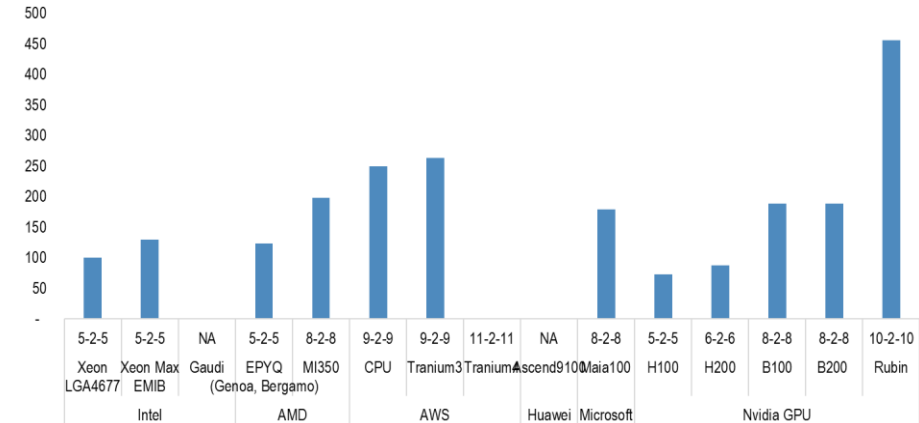
SAP size by product (Xeon LGA4677=100)
