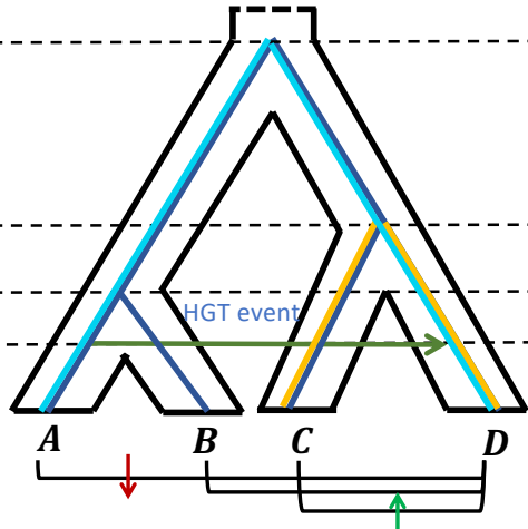
Species tree
