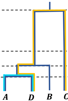
Gene tree with HGT
