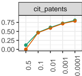
Resolution value
