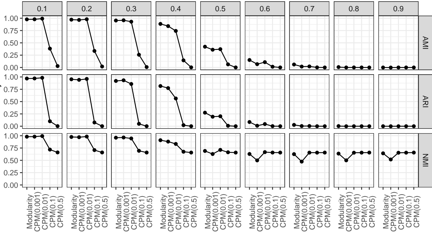
Accuracy
