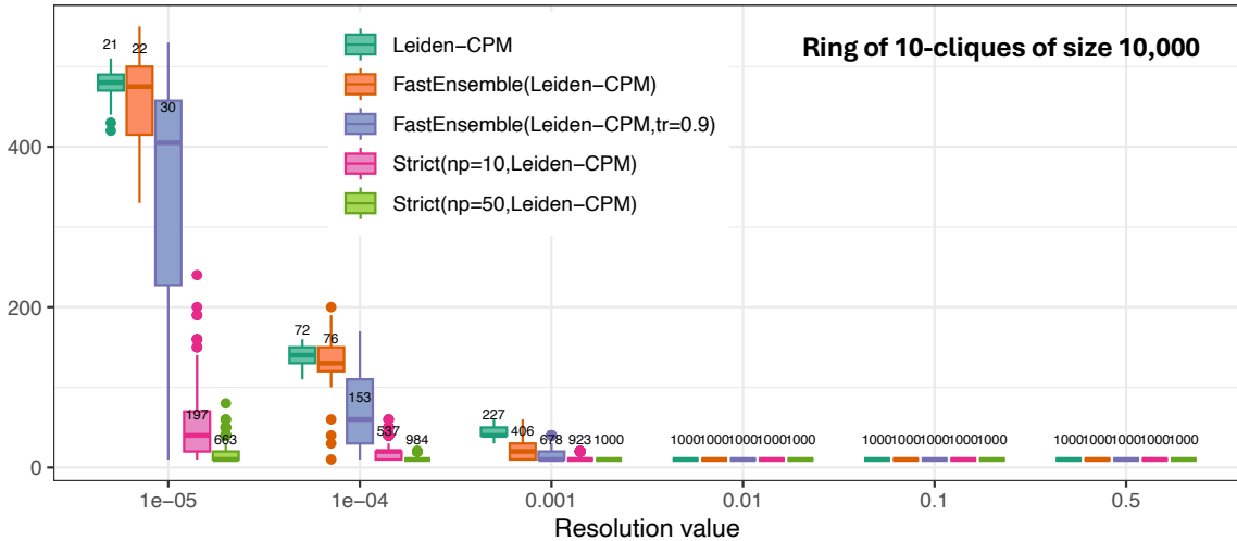
Cluster size distribution
