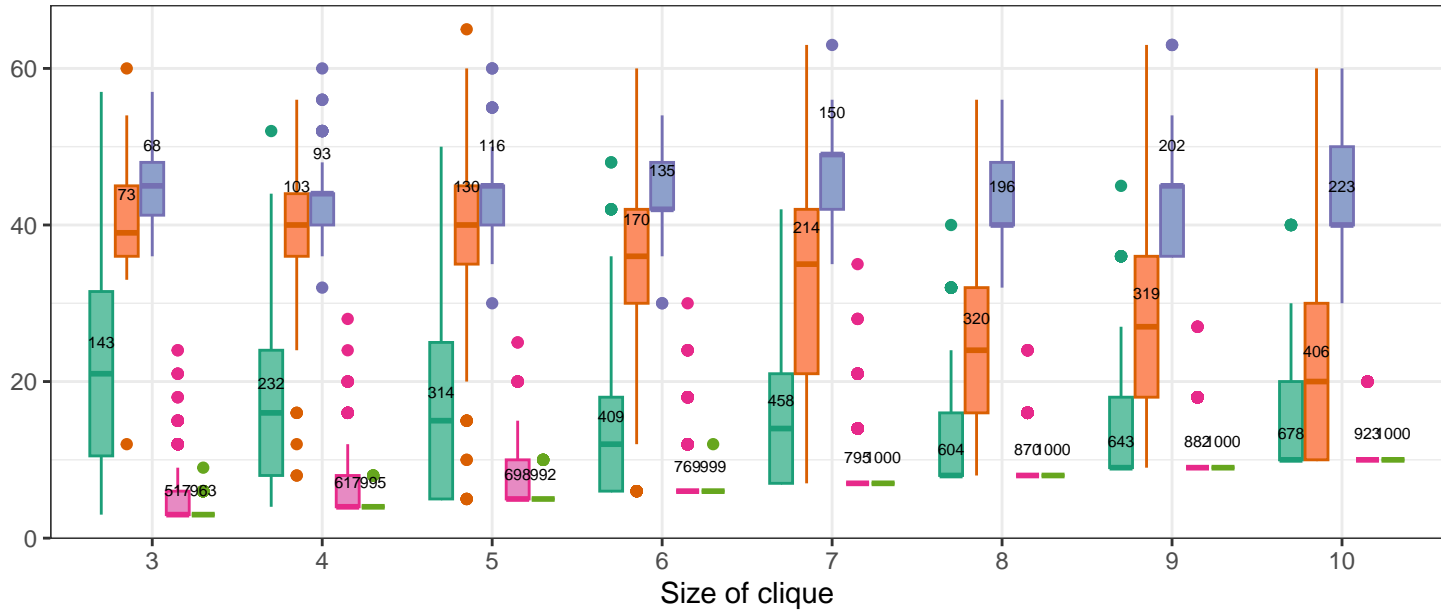
Cluster size distribution
