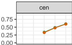
Modularity score
