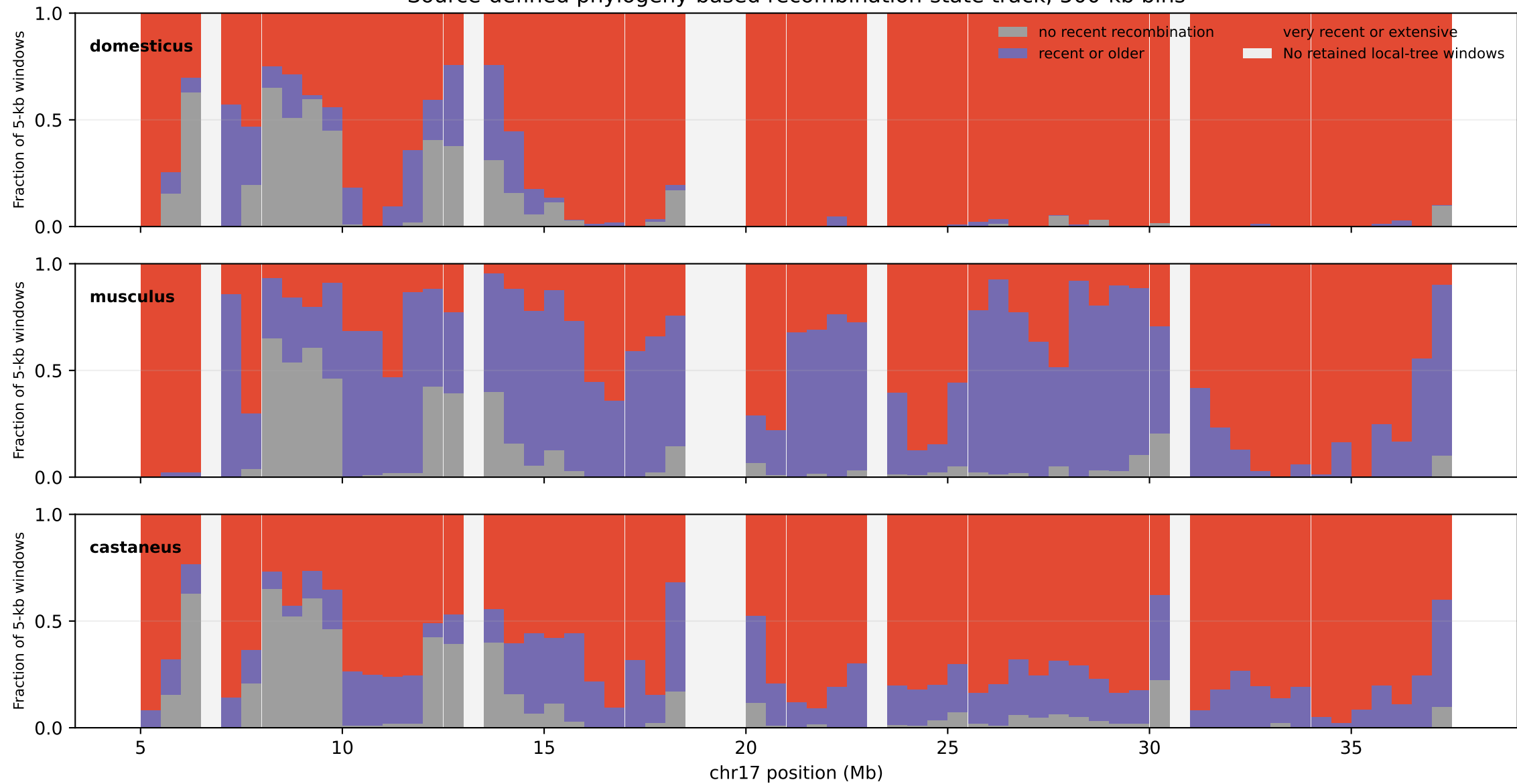
Source-defined phylogeny-based recombination-state track; 500-kb bins
