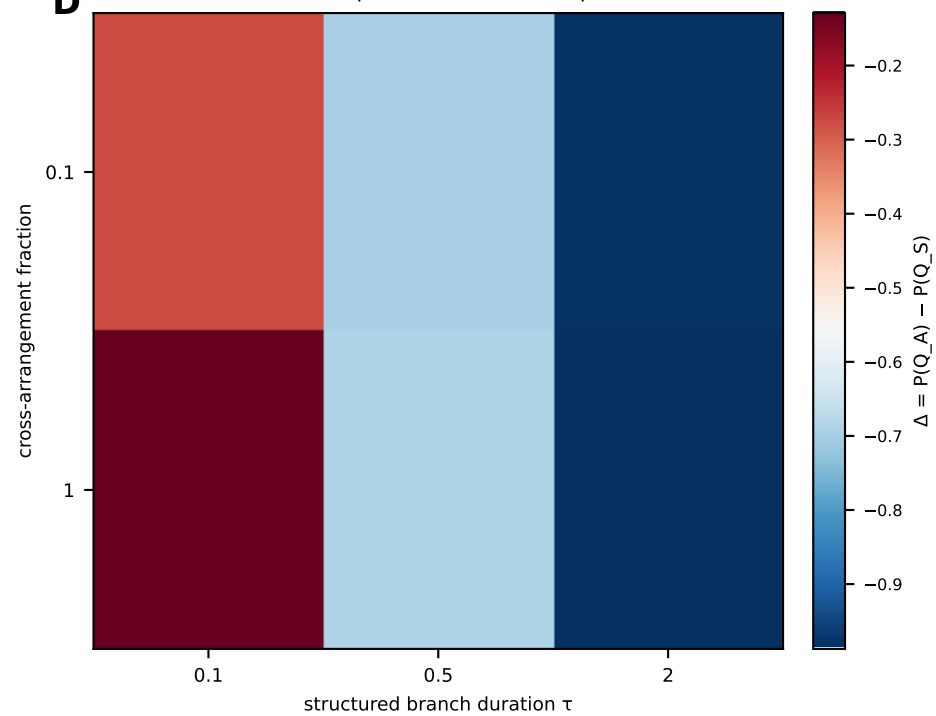
Unconditional quartet bias across a pilot slice
