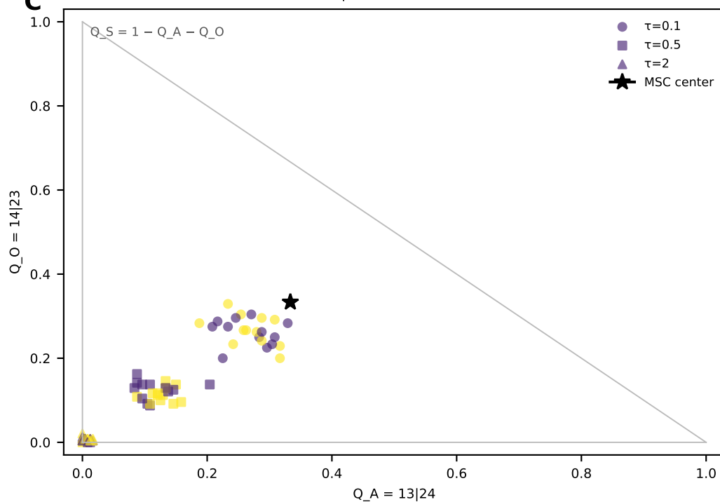
Pilot quartet distributions
