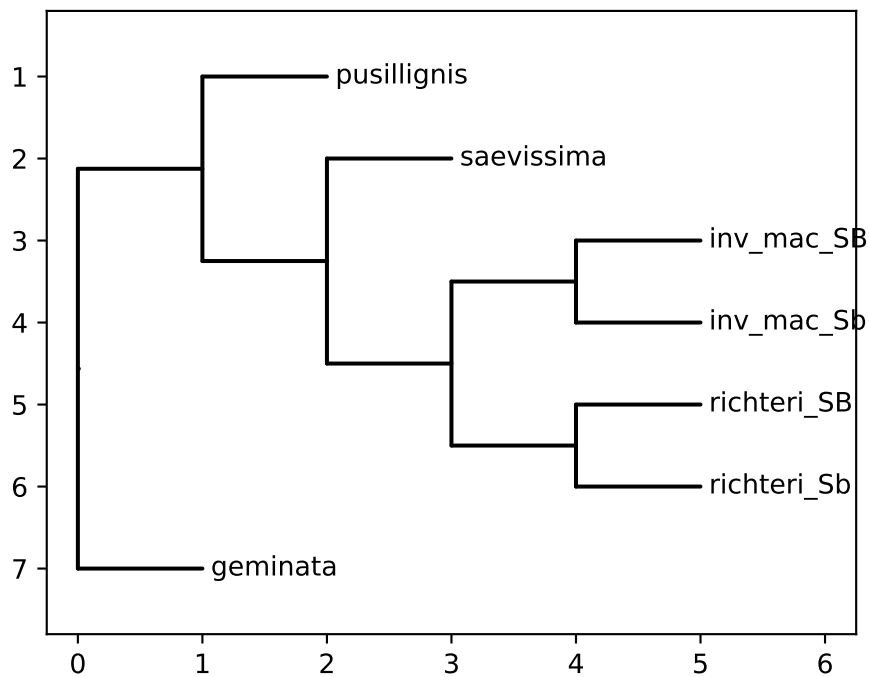
C. all-window modal ASTRAL4
