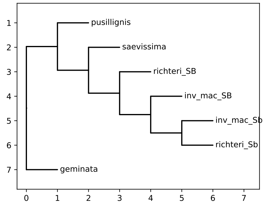
D. downweighting linked supergene windows
