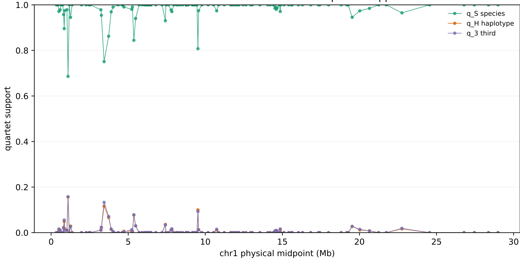
Fire ants chr1 TWISST-derived focal quartet support
