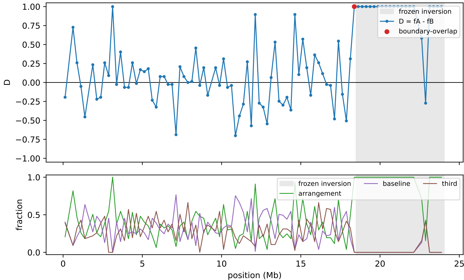
Atlantic cod LG02: local quartet topology track
