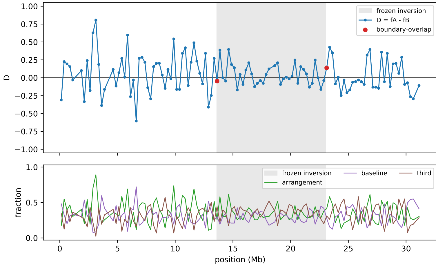
Atlantic cod LG07: local quartet topology track
