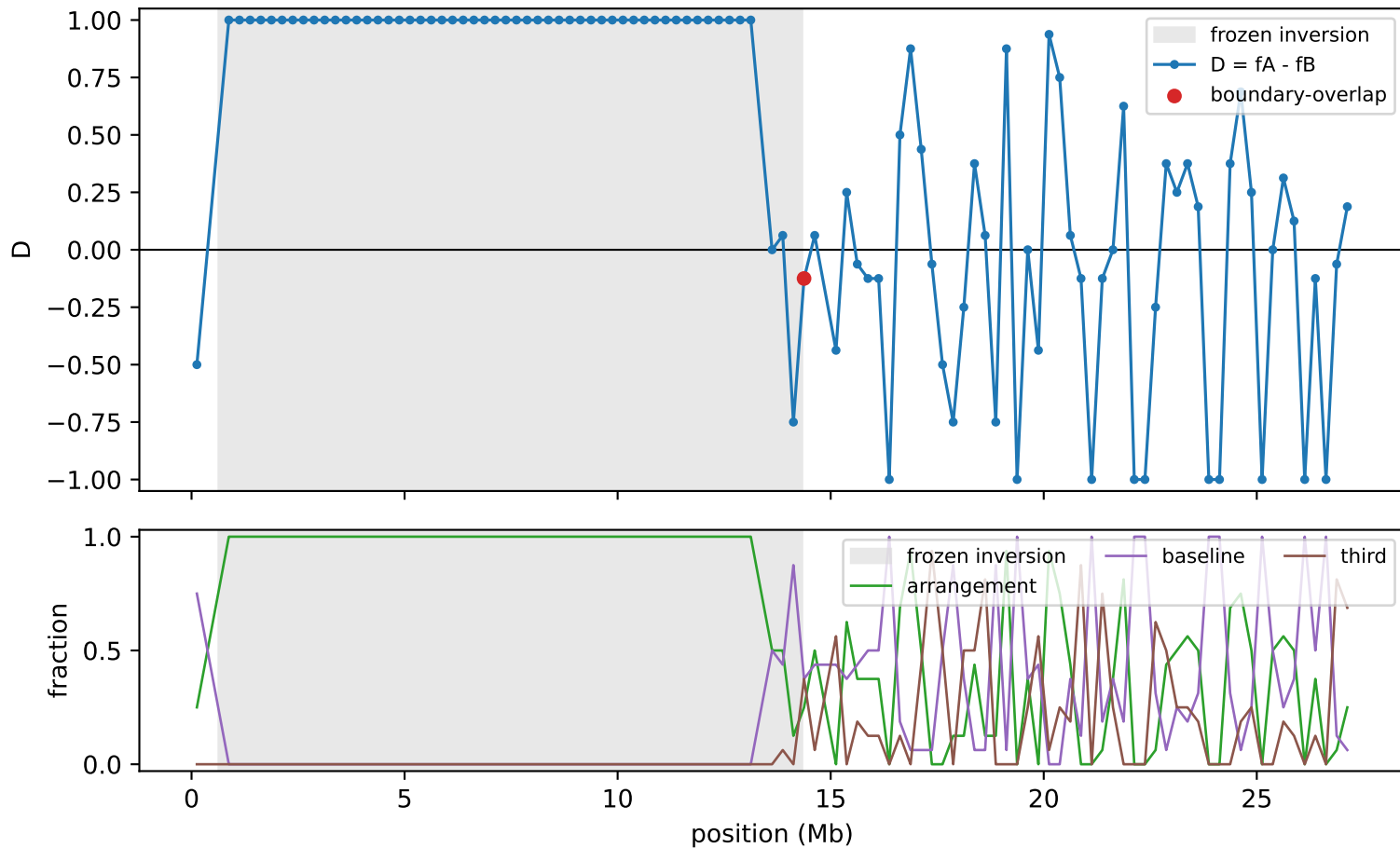
Atlantic cod LG12: local quartet topology track
