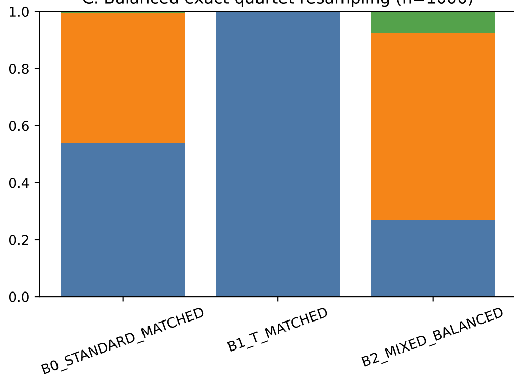
C. Balanced exact quartet resampling (n=1000)
