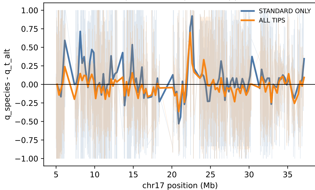
C. Balanced exact quartet resampling (n=1000)
