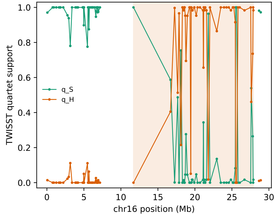
A. Local quartet support
