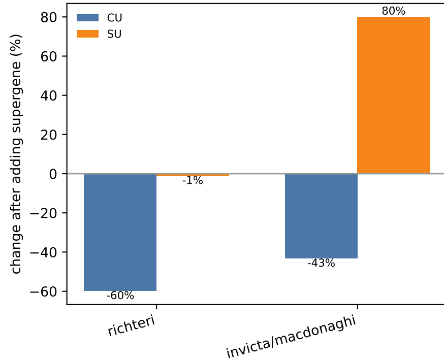
C. Fixed-topology branch lengths
