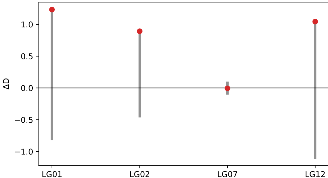
Stage 4B observed effects and circular-shift null ranges
