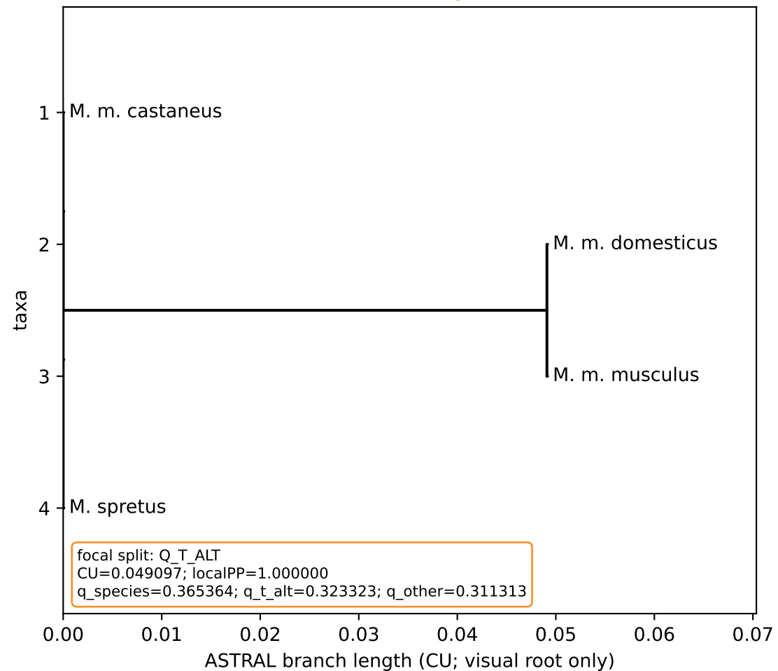
ALL standard + pseudo-t
