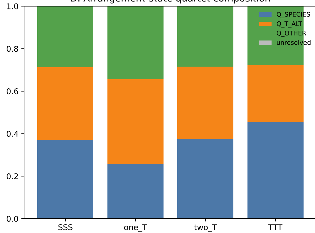
D. Arrangement-state quartet composition
