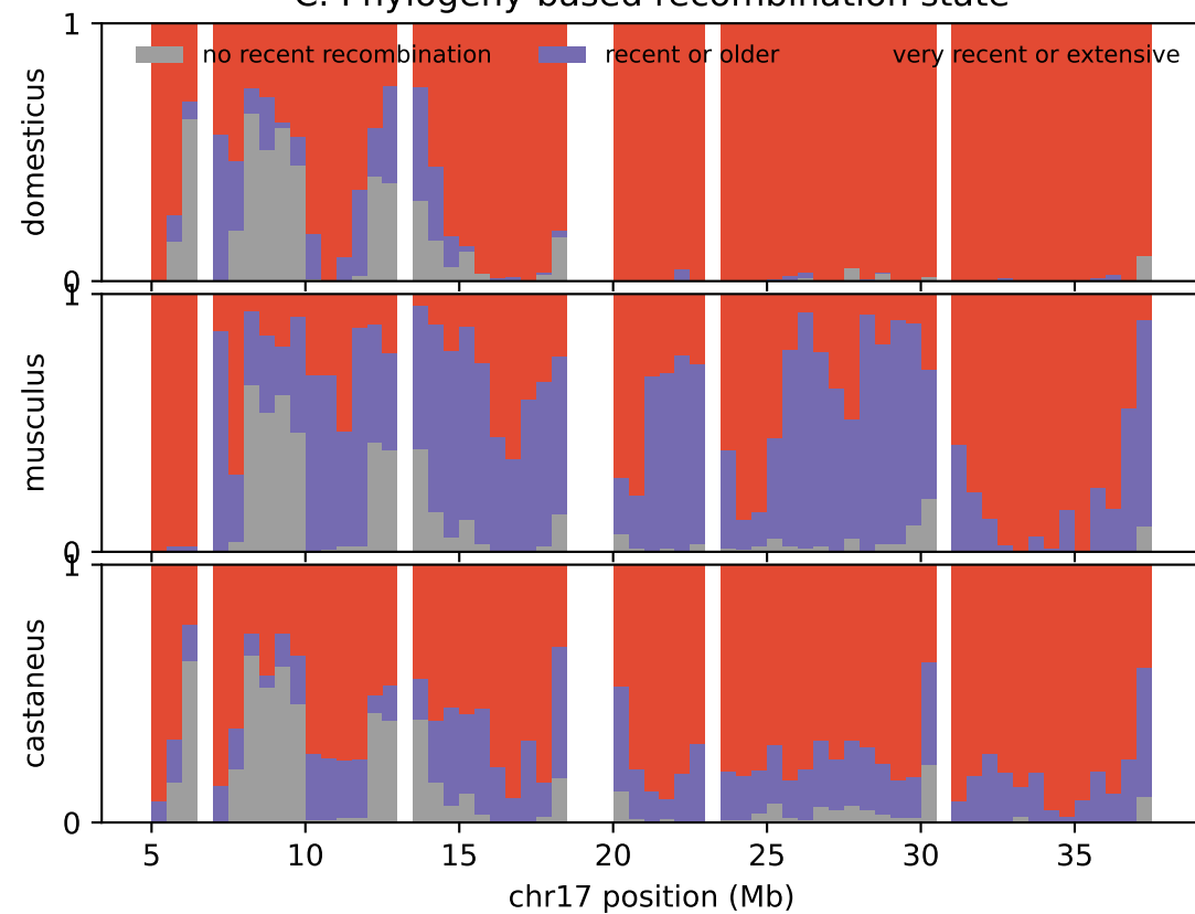
C. Phylogeny-based recombination state
