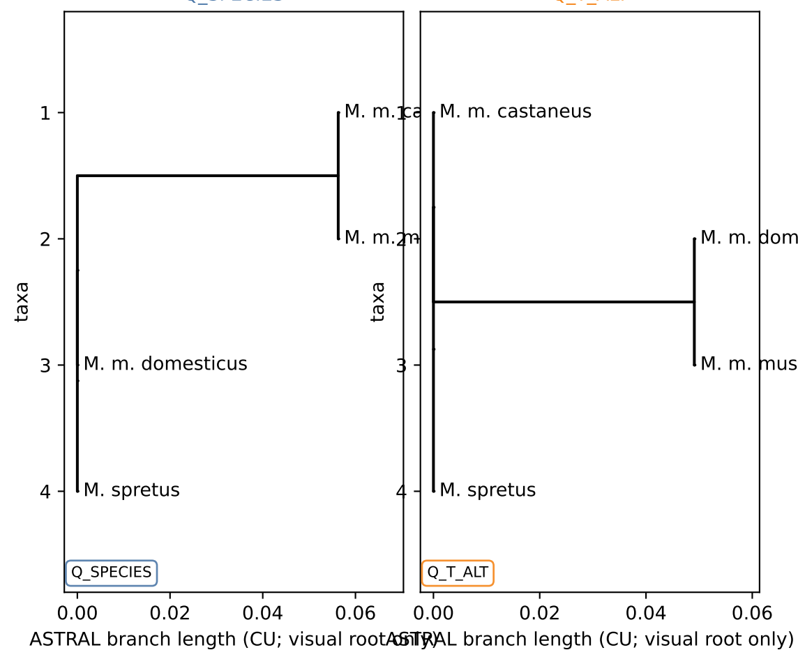
A. STANDARD Q_SPECIES
