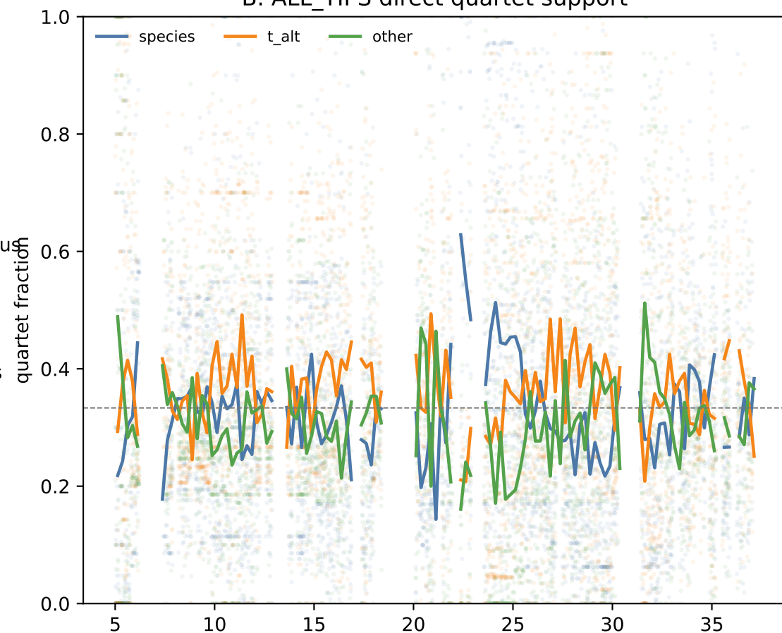
B. ALL_TIPS direct quartet support
