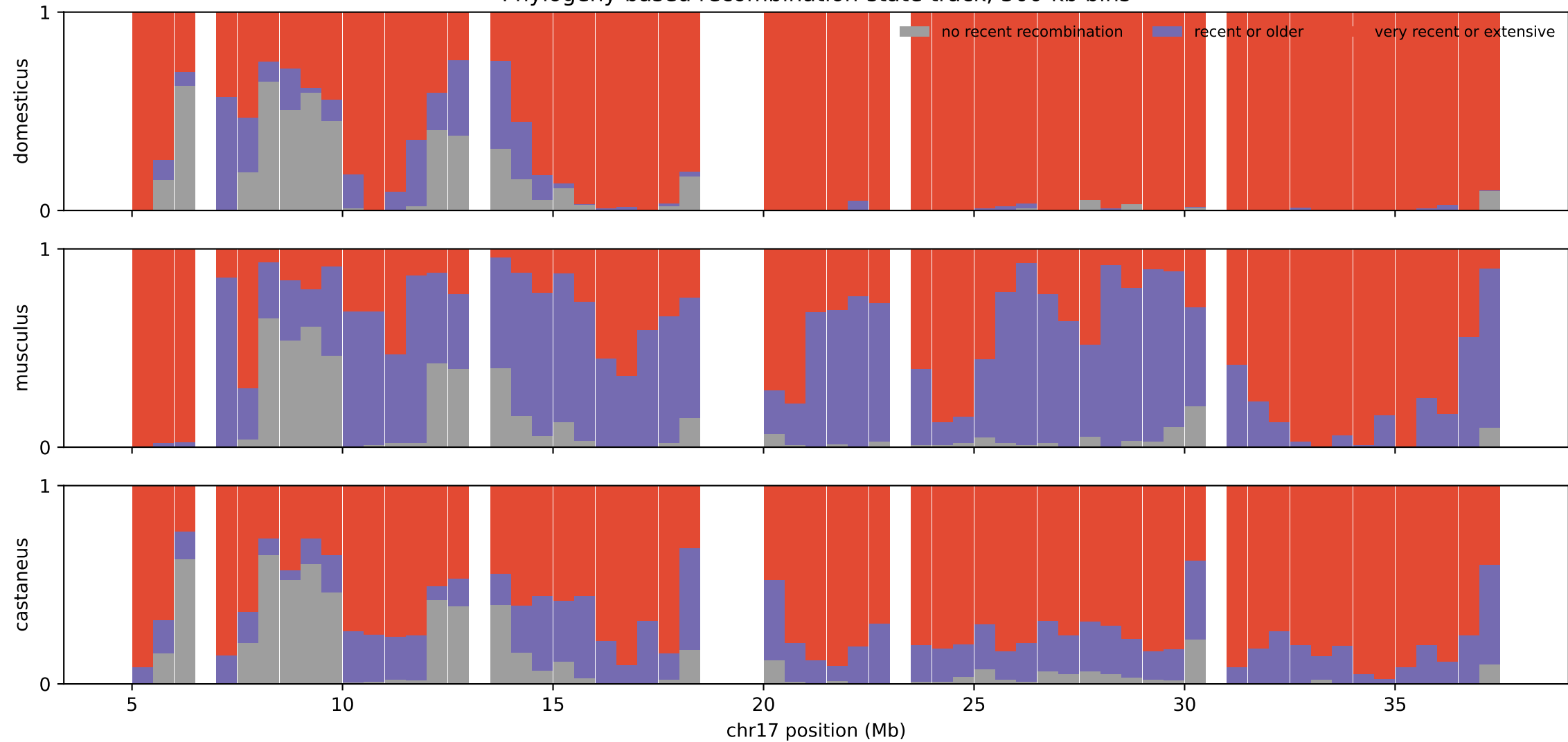
Phylogeny-based recombination-state track; 500-kb bins
