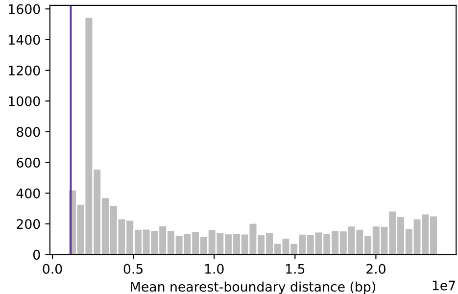
pooled
