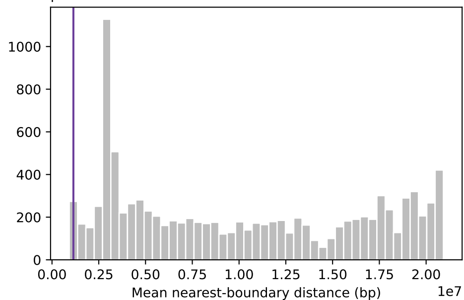
pooled
