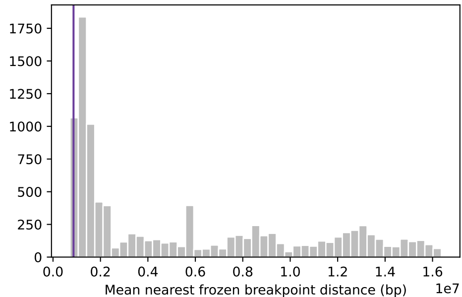
pooled
