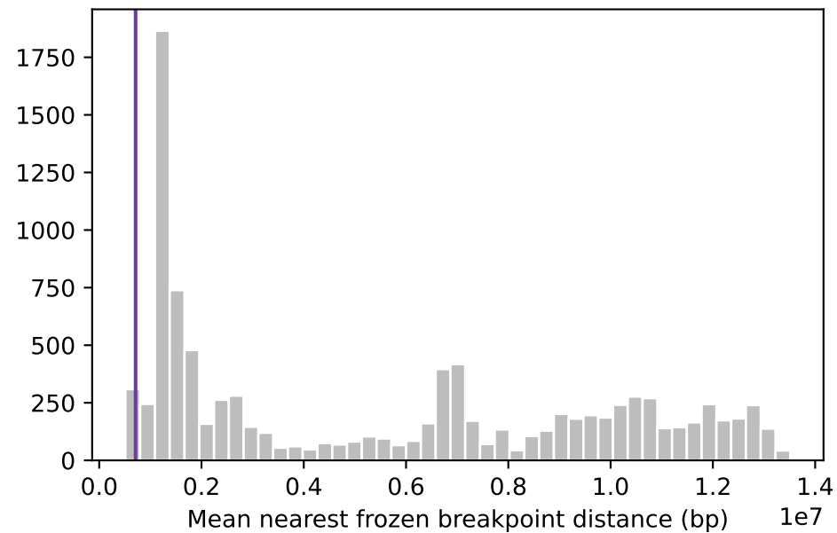
pooled
