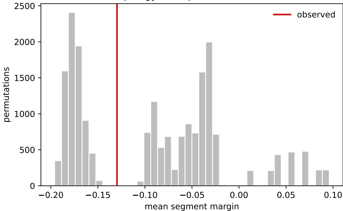
Topology-label permutation null
