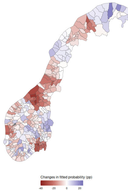
Figure 6: Geographic variation in the difference in the fitted proportion of uncertain-onset stroke between post treatment pathways for stroke minus the pre-treatment pathways
