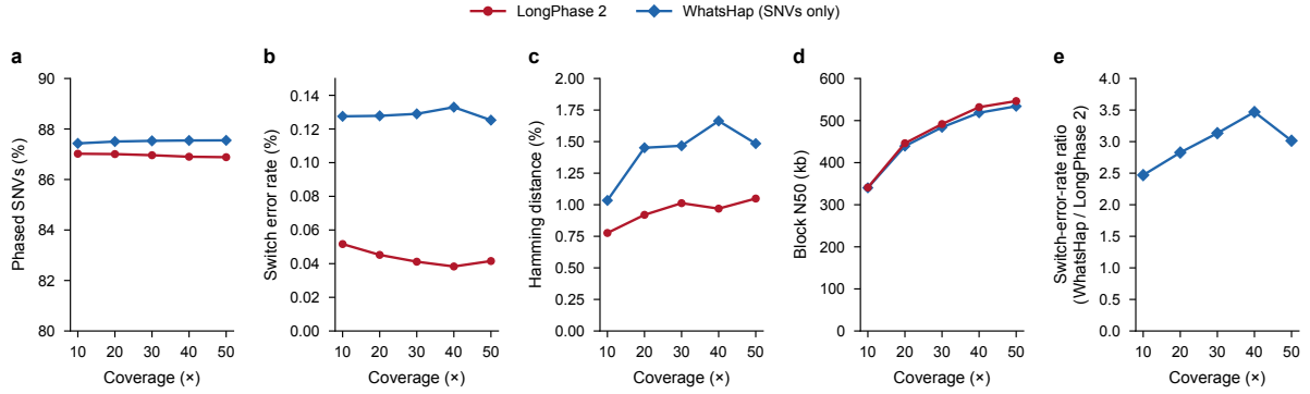
Figure 5: Phasing of PacBio HiFi data compared with WhatsHap. HG002 PacBio HiFi (Revo) reads down-sampled to 10–50 \times , one replicate per coverage[ state whether one call set was used for every coverage ]; SNV-only phasing scored against v5.0q; LongPhase 2 uses the network trained on nanopore data. Panels as in Fig. 2a–e. a , Fraction of benchmark heterozygous SNVs phased. b , Switch error rate. c , Block-wise Hamming distance. d , Phase-block N50. e , Switch error rate of WhatsHap divided by that of LongPhase 2.
