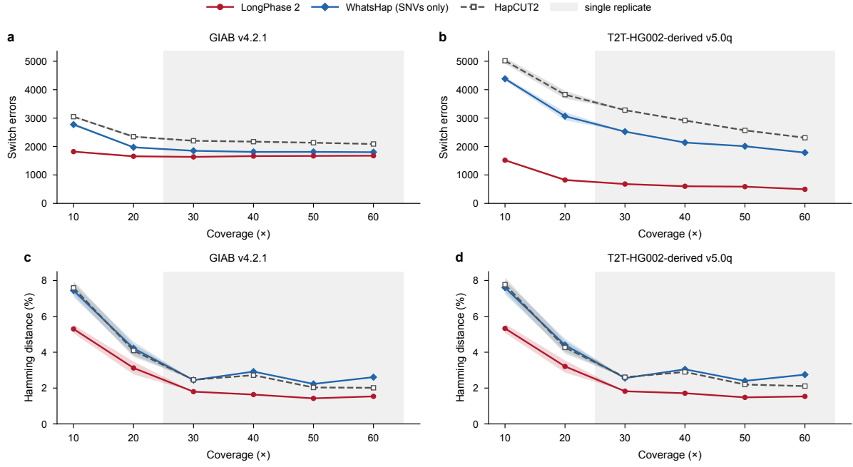
Figure 3: The same phased VCFs scored against GIAB v4.2.1 and the T2T-HG002-derived v5.0q benchmark. SNV-only phasing of HG002 nanopore R10.4.1 data; replicates and shading as in Fig. 2. a,b , Genome-wide switch errors under v4.2.1 ( a ) and v5.0q ( b ), on a shared axis. c,d , Hamming distance under v4.2.1 ( c ) and v5.0q ( d ).
