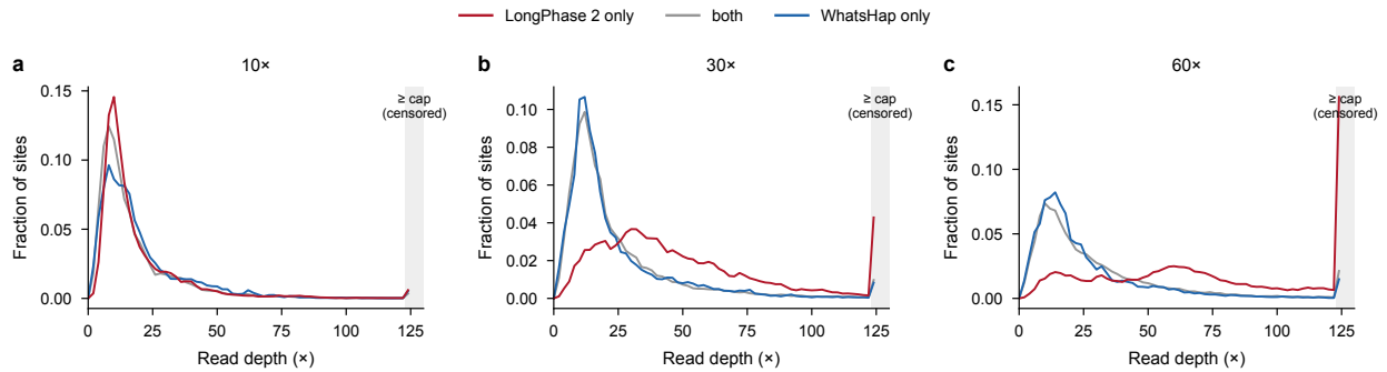
Supplementary Fig. 12: Read depth at heterozygous SNV calls left unphased by LongPhase 2, by WhatsHap or by both. HG002 nanopore R10.4.1 data, replicate 1, at 10 \times ( a ), 30 \times ( b ) and 60 \times ( c ); 2 \times bins. The grey bin collects every site at or above the depth cap of the variant caller (about 125 \times ), whose true depth is censored. Sets as in Fig. 6a.
