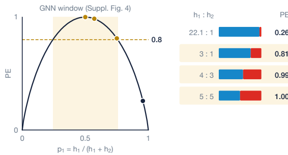
Supplementary Fig. 2: Pairwise allele support, weighted voting and phasing entropy. a , Between two variants u and v the reads accumulate four weights ( w_{rr}, w_{ra}, w_{ar}, w_{aa} ), each read adding 1 when both bases have quality \geq Q12 and 0.1 otherwise. P = w_{rr} + w_{aa} and Q = w_{ra} + w_{ar} are the supports for the two possible pairings and s = \min(P, Q) / \max(P, Q) their ambiguity. b , The pair votes for the better-supported pairing: at weight 20 when s \leq 0.1 with P + Q \geq 1 or, irrespective of s , when one pairing has less than 1 unit of support and the other at least 1; at weight 1 otherwise; and not at all when s > 0.7 (0.3 for SNV-5mC pairs, which also cast no vote when P + Q < 1 ). A voting variant that is a tandem-repeat indel votes at weight 0.1. The vote names a haplotype for v relative to the haplotype already assigned to u . c , Variant v receives weighted votes from up to k = 35 upstream variants that share a read with it, at any distance; line thickness encodes vote weight. The weighted totals h_1 and h_2 decide the haplotype; a tie opens a new phase block. d , Guard against a single erroneous ultra-long read: among the votes received by v , those resting on a single read ( P + Q \leq 1 , amber) are counted, and if more than three exist, h_1 and h_2 are recomputed from the votes with s < 0.2 , weight \geq 1 and a non-indel voter only. e , Phasing entropy of the vote totals, PE = -\sum_i p_i \log_2 p_i with p_i = h_i / (h_1 + h_2) , as a function of the vote split (left) and for four examples (right); values \geq 0.8 (shaded) open a window for the neural network (Supplementary Fig. 4). PE, h_1 and h_2 are written to the VCF as INFO/PE, INFO/H1 and INFO/H2. f , Block formation. Variants are visited in coordinate order; a variant whose next heterozygous variant lies more than 300 kb away ( -distance ) is skipped and casts no votes, a variant that receives no informative vote or a tie (amber) starts a new phase set when it lies beyond the last position reached by an accepted edge and is otherwise left unphased, and blocks holding a single variant are dropped (grey). Haplotype labels propagate along the block as the phased genotypes 0|1 and 1|0; the phase set (PS) is the position of its first variant.
