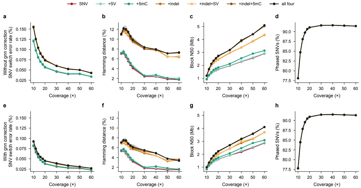
Supplementary Fig. 15: All co-phasing configurations across coverage. HG002 nanopore R10.4.1 data; means of ten replicates with s.d. at 10–20 \times ; one down-sampling at 30–60 \times . Top row without, bottom row with GNN correction. a,e , SNV switch error rate. b,f , Hamming distance (over SNVs and indels where indels are phased). c,g , Block N50. d,h , Fraction of benchmark heterozygous SNVs phased. Values in Supplementary Table 10.
