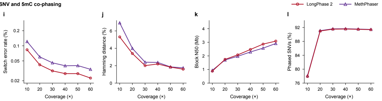
Figure 2: LongPhase 2 compared with other phasers for each type of phasing evidence. HG002 nanopore R10.4.1 reads down-sampled to 10–60×; identical variant calls for every tool, scored against the T2T-HG002-derived v5.0q benchmark. Values at 10–20× are means of ten down-sampling replicates with the s.d. as a light band; values at 30–60× come from one down-sampling (Methods). Columns show the switch error rate (log scale), block-wise Hamming distance, phase-block N50 and the fraction of benchmark heterozygous variants phased. a–d , SNV phasing compared with WhatsHap and HapCUT2. e–h , SNV and indel co-phasing compared with WhatsHap. In e , solid lines score consecutive SNV pairs and dotted lines consecutive pairs that include an indel; f and h refer to indels (Supplementary Table 14). i–l , SNV and 5mC co-phasing compared with MethPhaser, replicate 1; MethPhaser was given the SNV-only output of LongPhase 2 without GNN correction (Methods).
