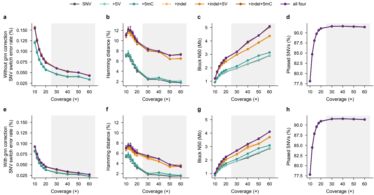
Supplementary Fig. 15: All co-phasing configurations across coverage. HG002 nanopore R10.4.1 data; means of ten replicates with s.d. at 10–20×; shaded, single replicate. Top row without, bottom row with GNN correction. a,e , SNV switch error rate. b,f , Hamming distance (over SNVs and indels where indels are phased). c,g , Block N50. d,h , Fraction of benchmark heterozygous SNVs phased. Values in Supplementary Table 10.
