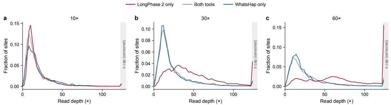
Supplementary Fig. 12: Read depth at heterozygous SNV calls left unphased by LongPhase 2, by WhatsHap or by both. HG002 nanopore R10.4.1 data, replicate 1, at 10× ( a ), 30× ( b ) and 60× ( c ); 2× bins. The grey bin collects every site at or above the depth cap of the variant caller (about 125×), whose true depth is censored. Sets as in Fig. 6a.
