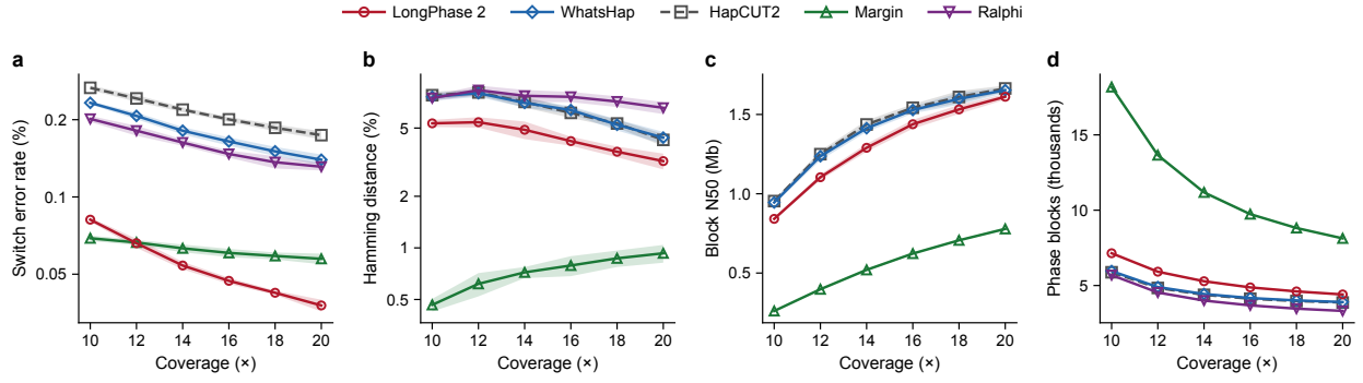
Supplementary Fig. 10: SNV-only phasing compared with Margin and Ralphi. HG002 nanopore R10.4.1 data at 10–20×, means of ten replicates with s.d., scored against v5.0q; LongPhase 2 with GNN correction. a , Switch error rate. b , Hamming distance. c , Block N50; Ralphi is omitted because its blocks sum to more than the autosome length. d , Number of phase blocks. Values in Supplementary Table 8.
