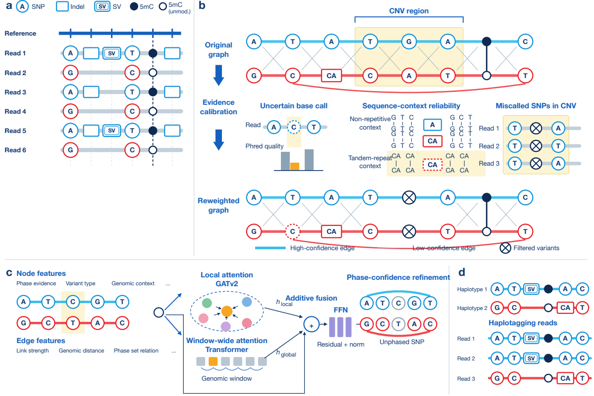
Figure 1: Overview of LongPhase 2. a , Heterogeneous molecular evidence (SNVs, small indels, structural variants and 5mC calls) from the same long reads is integrated into a single haplotype-resolution problem. b , Weighted phasing graph. Allele nodes are connected by read-supported edges; evidence is calibrated by base quality and sequence-context reliability (homopolymers, tandem repeats, miscalled heterozygous sites in copy-number-altered regions) before multi-neighbour haplotype voting and read-based correction. c , Optional uncertainty correction. Per-variant phasing entropy selects loci for a graph neural network that combines local attention over the phasing graph (GATv2) with window-wide attention (Transformer); variants predicted to be misphased are unphased and the affected phase set is split, preserving the genotype. d , Outputs: phased VCFs for all variant classes and haplotagged alignments.
