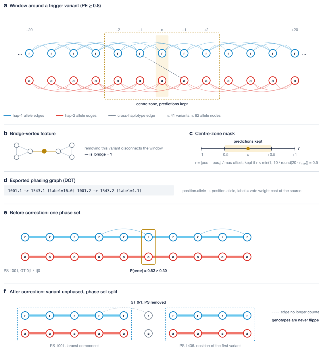
Supplementary Fig. 5: Window construction and phase-set update for the graph neural network. a , A window of \pm 20 variants (two allele nodes each) is opened around every phased variant with PE \geq 0.8 ; edges are the DOT edges with both endpoints in the window (blue and red arcs) plus self-loops; a dashed grey edge marks a cross-haplotype link. Predictions are read only in the central zone. b , Bridge-vertex feature: a variant whose removal disconnects the window graph. c , Definition of the central zone. A window holds at most 41 variants and 82 allele nodes (a 256-node cap exists but is never reached at the default window size); SNV, indel, SV and 5mC records are merged and sorted by position before nodes are created. The retained zone is the central half of the window's genomic span: variants no further from the trigger than half the largest trigger distance in the window. The same rule, with the same constant, defines which labelled nodes carried a training loss, and the zone scored at inference is the zone the network was trained on. Edges are the DOT edges with both endpoints in the window, symmetrized, plus one self-loop per node whose features are the mean over that node's incident edges. The predictions of the two allele nodes of a variant are averaged, and a variant covered by several windows receives the mean over those windows. d , The phasing graph that the module reads, shown in its DOT export format ( -dot ): one line per voting pair, source and target written as position.allele, and the vote weight accumulated at the source as the label. e , Phase-set update, before correction: a variant with predicted phase-error score \geq 0.30 (amber) inside a phase set. f , After correction the variant is written as an unphased genotype without PS; connectivity of the remaining variants is recomputed over the surviving DOT edges, the largest component keeps the original PS and every other component receives a new PS equal to the position of its first variant. Genotypes are never flipped.
