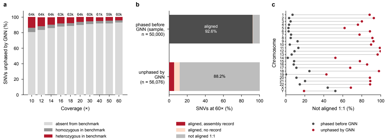
Supplementary Fig. 16: SNVs unphased by GNN correction. HG002 nanopore R10.4.1 data, SNV-only phasing, replicate 1. a , Classification against the v5.0q benchmark VCF; numbers above bars, total unphased. b , Status in the T2T-HG002 v1.1 assembly of the SNVs unphased at 60 \times and of a random sample of SNVs phased before GNN correction: inside or outside the regions where both assembled haplotypes align 1:1 to GRCh38, and, inside, whether an assembly variant record starts at the same coordinate. c , Per chromosome, fraction of each set outside the 1:1 alignment. Values in Supplementary Table 12. [Rebuild from one site-level table (autosomes only, control excluding removed sites, allele-aware assembly comparison) before submission.]
