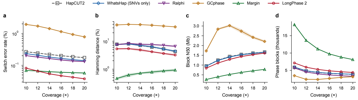
Supplementary Fig. 10: SNV-only phasing compared with Margin, Ralphi and GCphase. HG002 nanopore R10.4.1 data at 10–20 \times , means of ten replicates with s.d., scored against v5.0q; LongPhase 2 with GNN correction. a , Switch error rate. b , Hamming distance. c , Block N50; Ralphi is omitted because its blocks sum to more than the autosome length. d , Number of phase blocks. Values in Supplementary Table 8.
