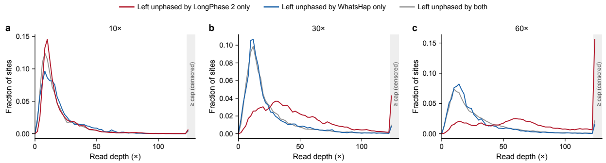
Supplementary Fig. 12: Read depth at heterozygous SNV calls left unphased by LongPhase 2 only, by WhatsHap only or by both. HG002 nanopore R10.4.1 data, replicate 1, at 10x (a), 30x (b) and 60x (c); 2x bins. The grey bin collects every site at or above the depth cap of the variant caller (about 125x), whose true depth is censored. Sets as in Supplementary Table 17.
