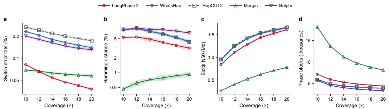
Supplementary Fig. 9: SNV-only phasing compared with Margin and Ralphi. HG002 nanopore R10.4.1 data at 10–20 \times , means of ten replicates with s.d., scored against v5.0q; LongPhase 2 with GNN correction. a , Switch error rate. b , Hamming distance. c , Block N50; Ralphi is omitted because its blocks sum to more than the autosome length. d , Number of phase blocks. Values in Supplementary Table 8.
