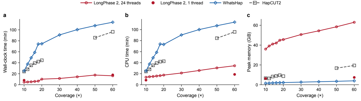
Supplementary Fig. 10: Runtime and peak memory of SNV-only phasing. HG002 nanopore R10.4.1 data, replicate 1, on the workstation described in Methods; values in Supplementary Table 16. LongPhase 2 includes GNN correction and was run with 24 threads at every coverage and on one thread at 10 and 60x; WhatsHap and HapCUT2 run on one thread. HapCUT2 times are not available at 30 and 40x. a , Wall-clock time. b , CPU time (user plus system). c , Peak resident memory.
